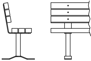
ALTERNATIVE BENCH WITH 3" X 4" BOARDS
