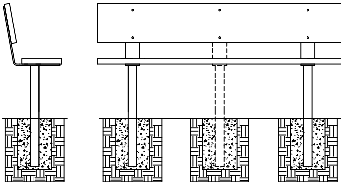
ALTERNATIVE BENCH WITH 3" X 4" BOARDS
